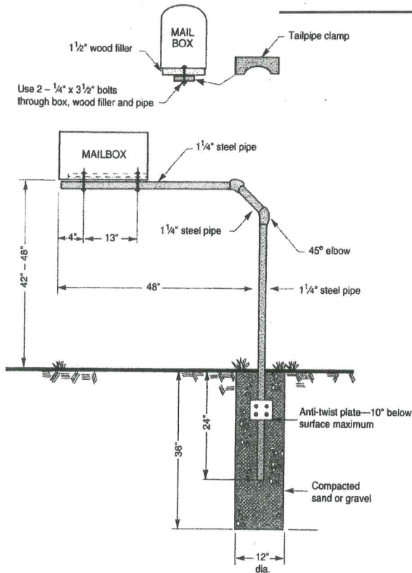
Example of a steel pipe cantilever mailbox support
