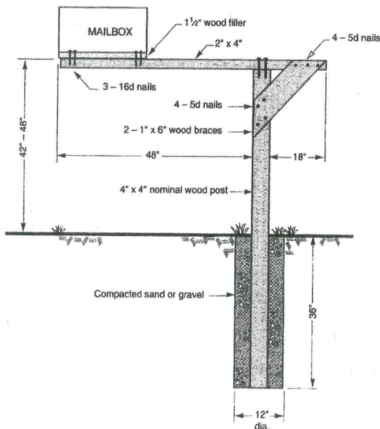
Example of a wood cantilever mailbox support
